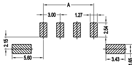
PCB LAYOUT(Tolerance:±0.05)
