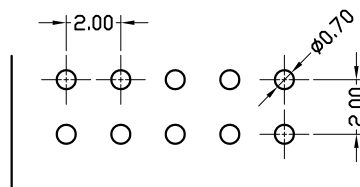
P. C. B LAYOUT
