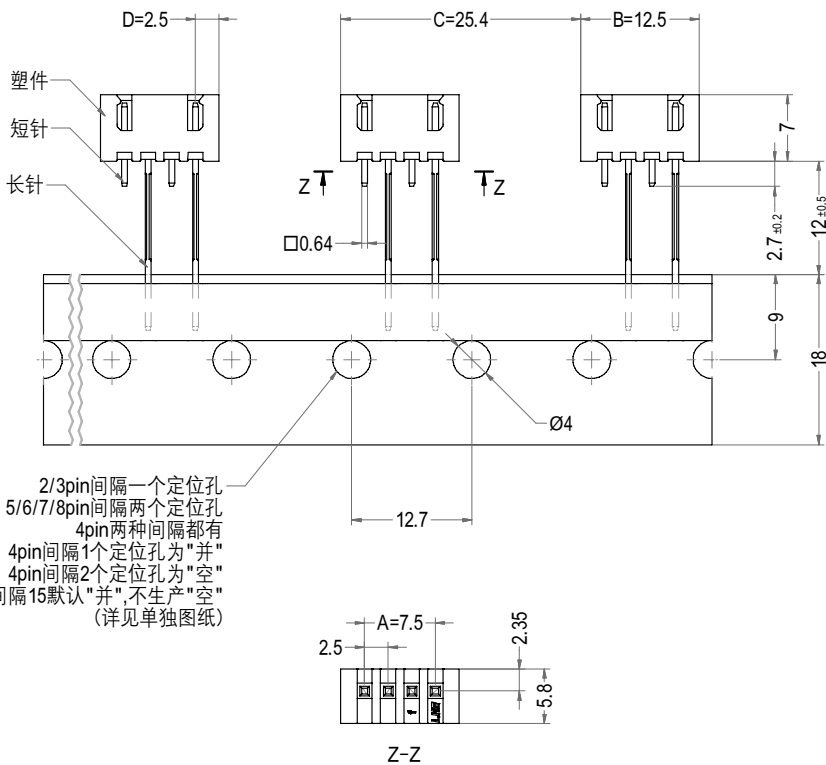
XH-4A(1.3长针)编带装(空)
